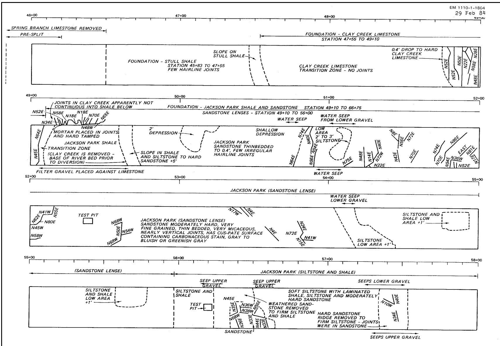
Figure B-8. Foundation map for earth dam impervious core on sedimentary rocks (note: 1 ft = 0.3 m)
