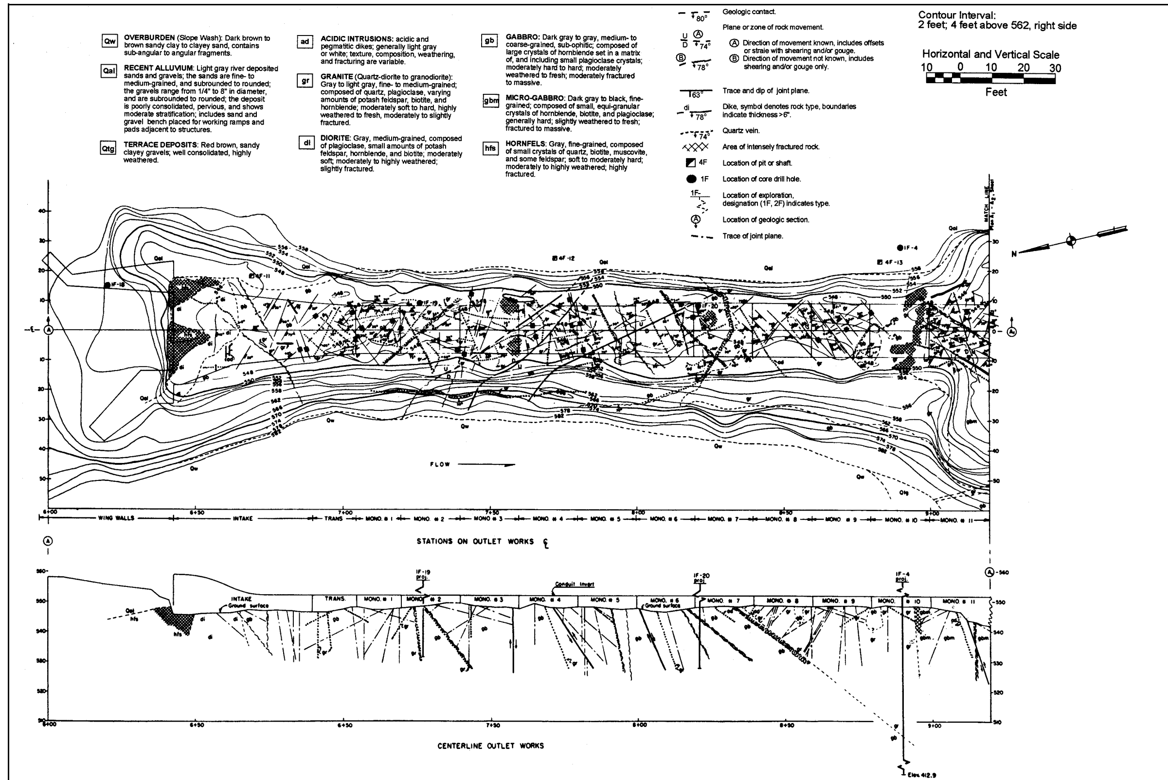
Figure B-2. Example of a foundation map for concrete structure on metavolcanic and igneous rocks
