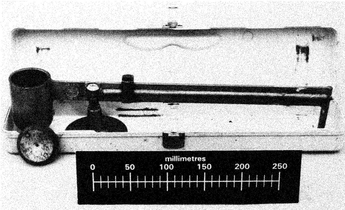
Figure 4-2. Mud balance for determining the density of drilling mud
