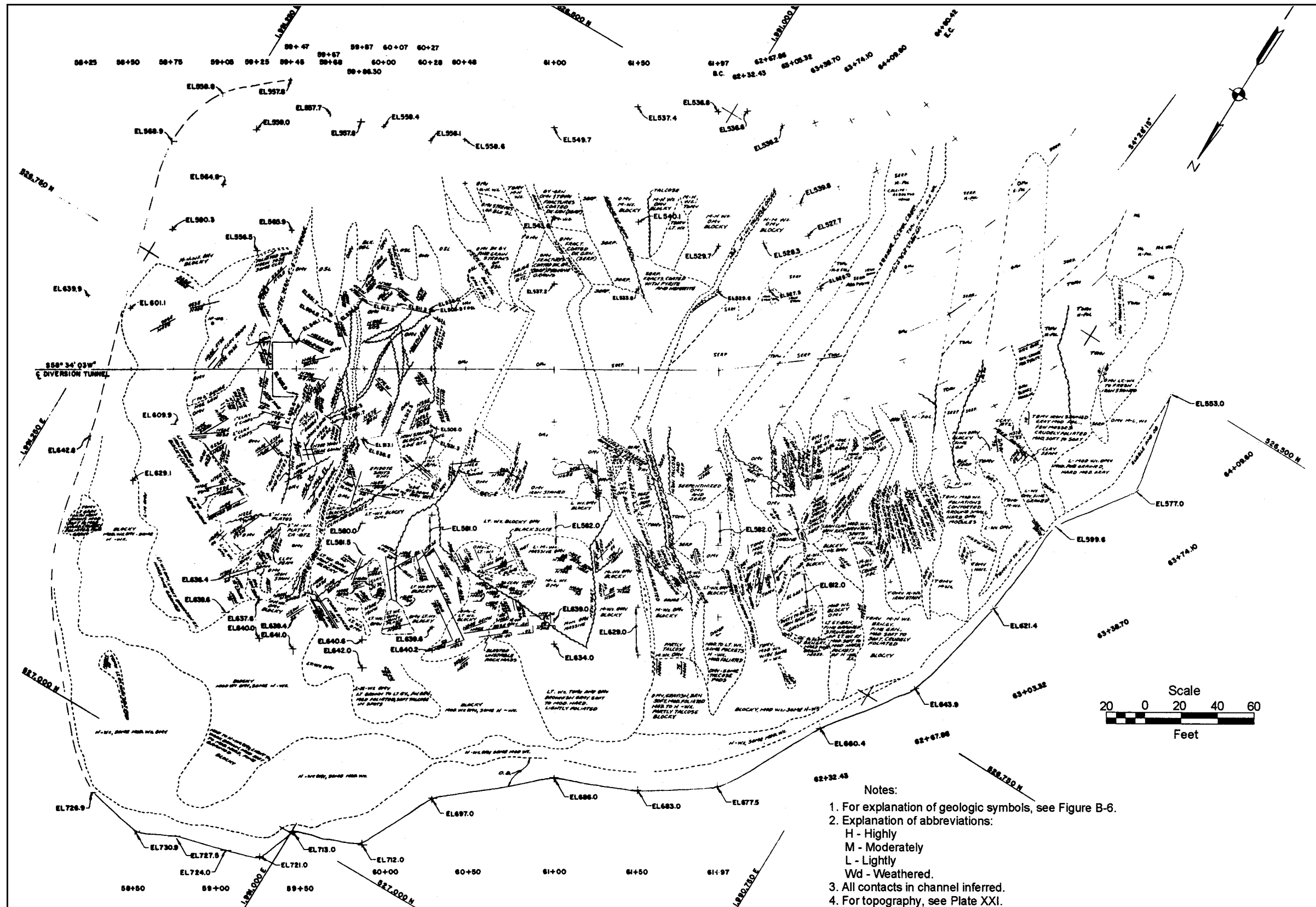
Figure B-5. Example of excavation map including area covered by Figure B-3
