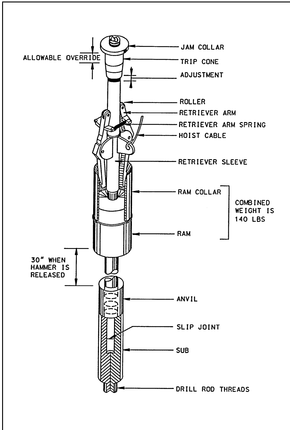
Figure G-2. Schematic drawing of the automatic trip hammer
