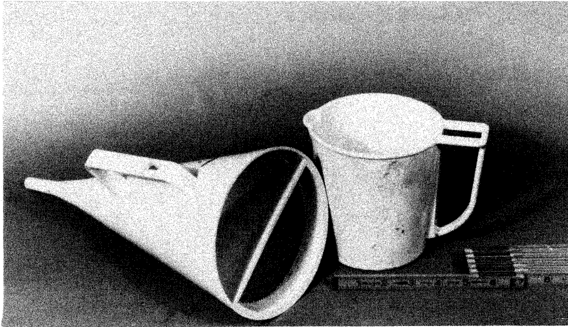
Figure 4-1. Photograph of a Marsh funnel and a one quart (0.95 dm 3 ) measuring cup for determining the viscosity of drilling mud
