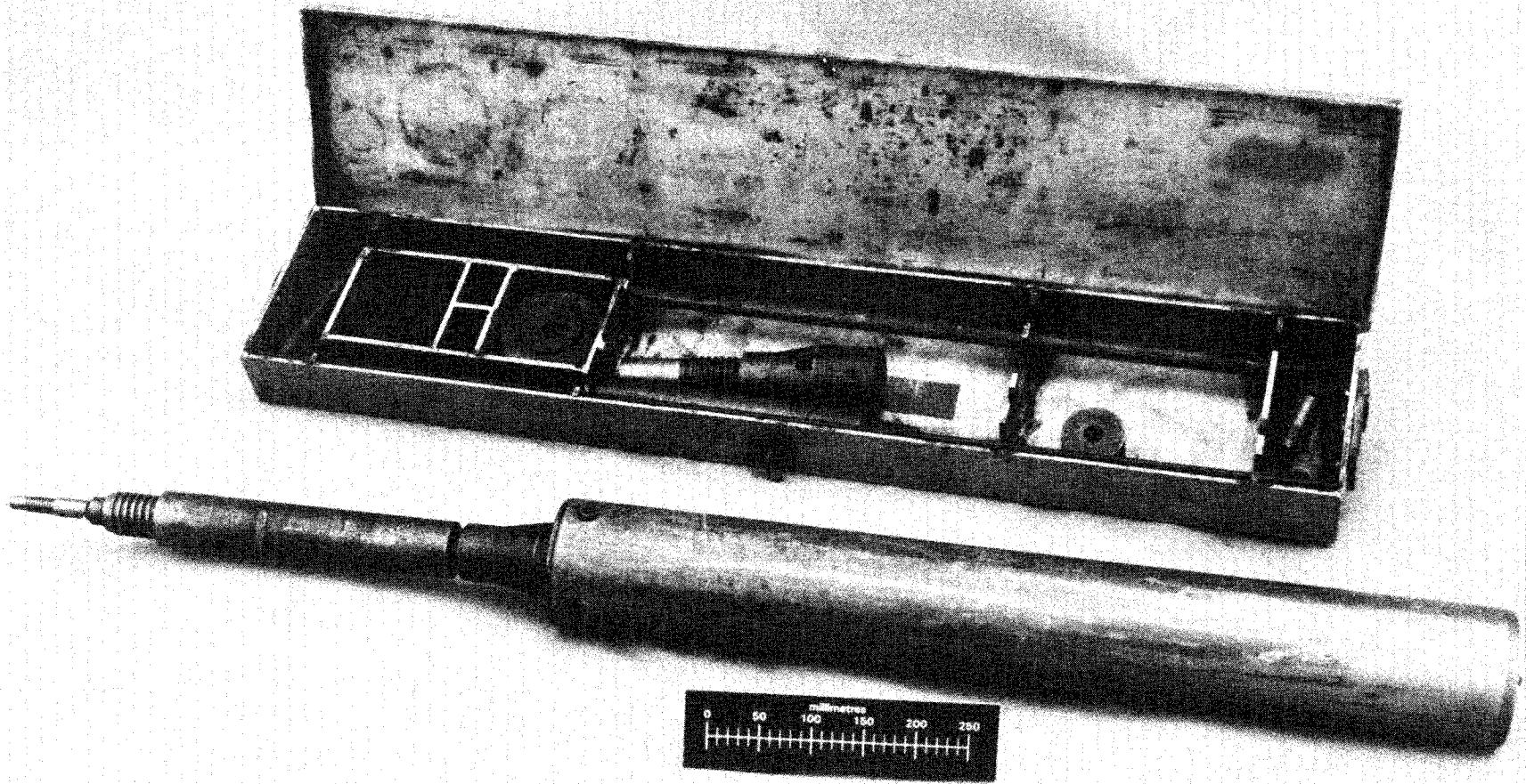
Figure 5-3. Photograph of the Hvorslev fixed-piston sampler
