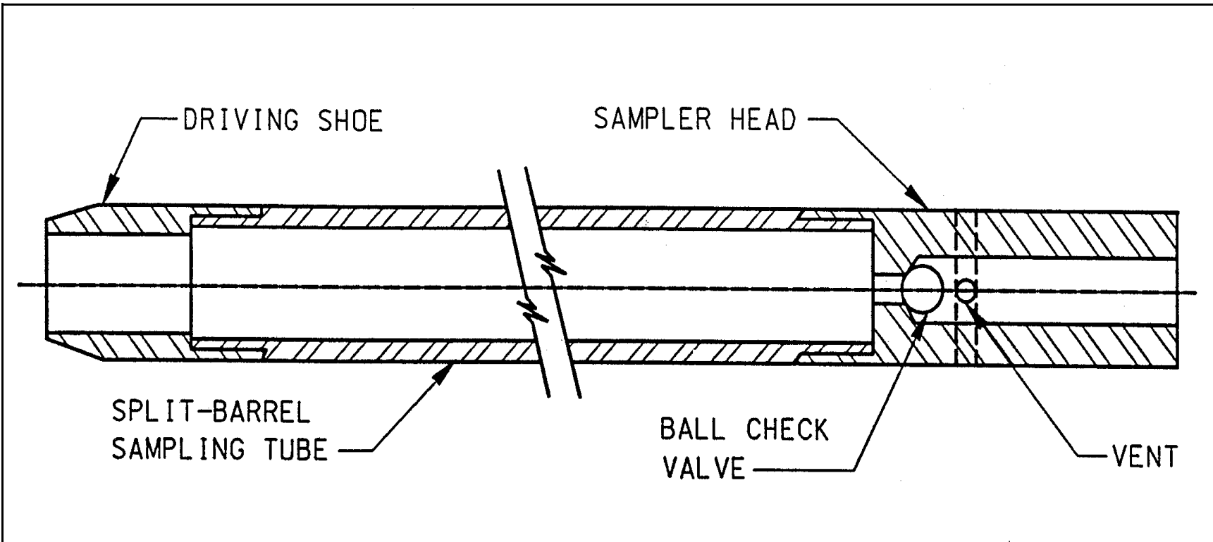
Figure G-4. Schematic drawing of the split-barrel sampler
