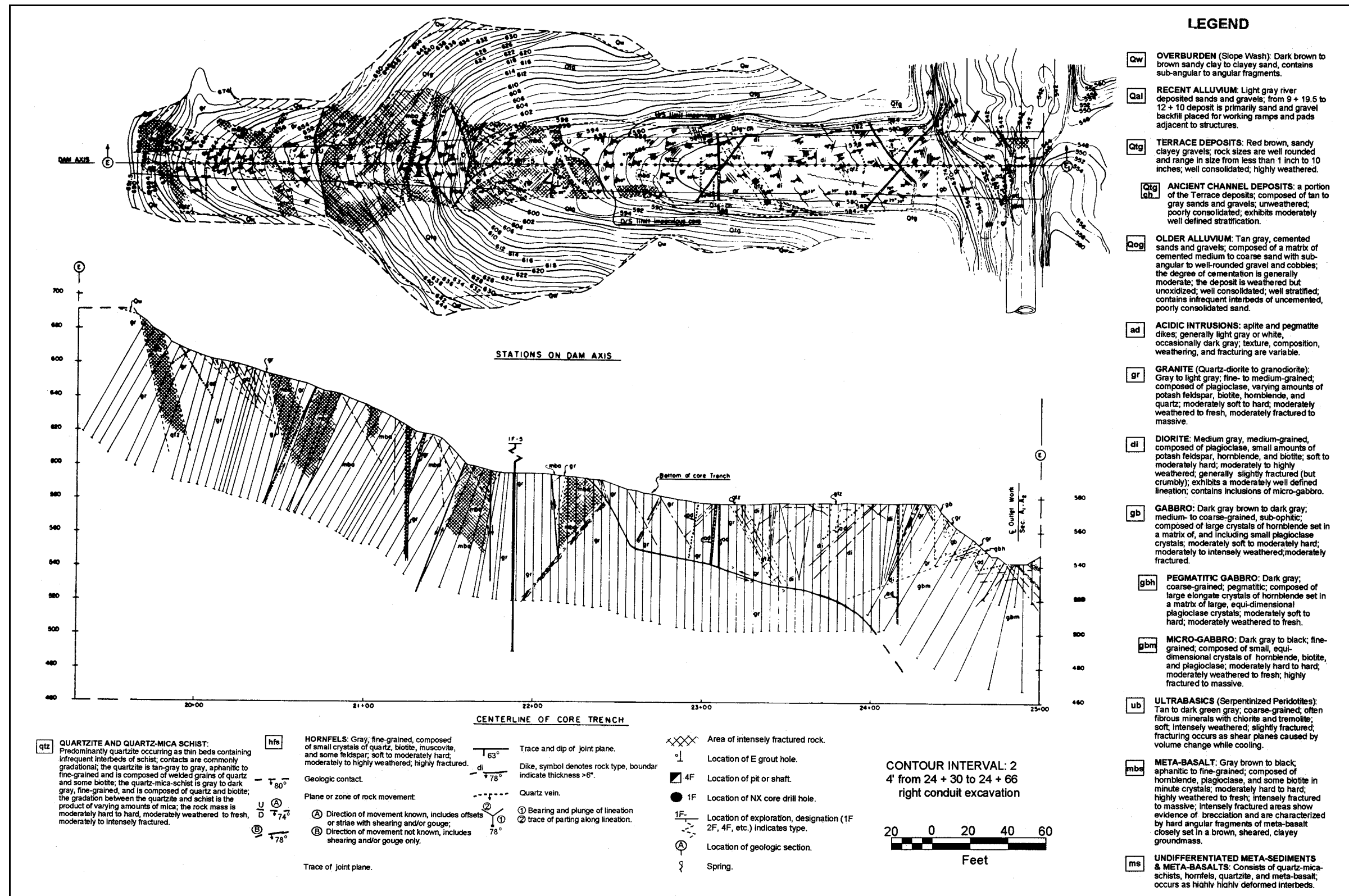
Figure B-6. Example of foundation map for earth dam impervious core on meta-volcanic and igneous rocks
