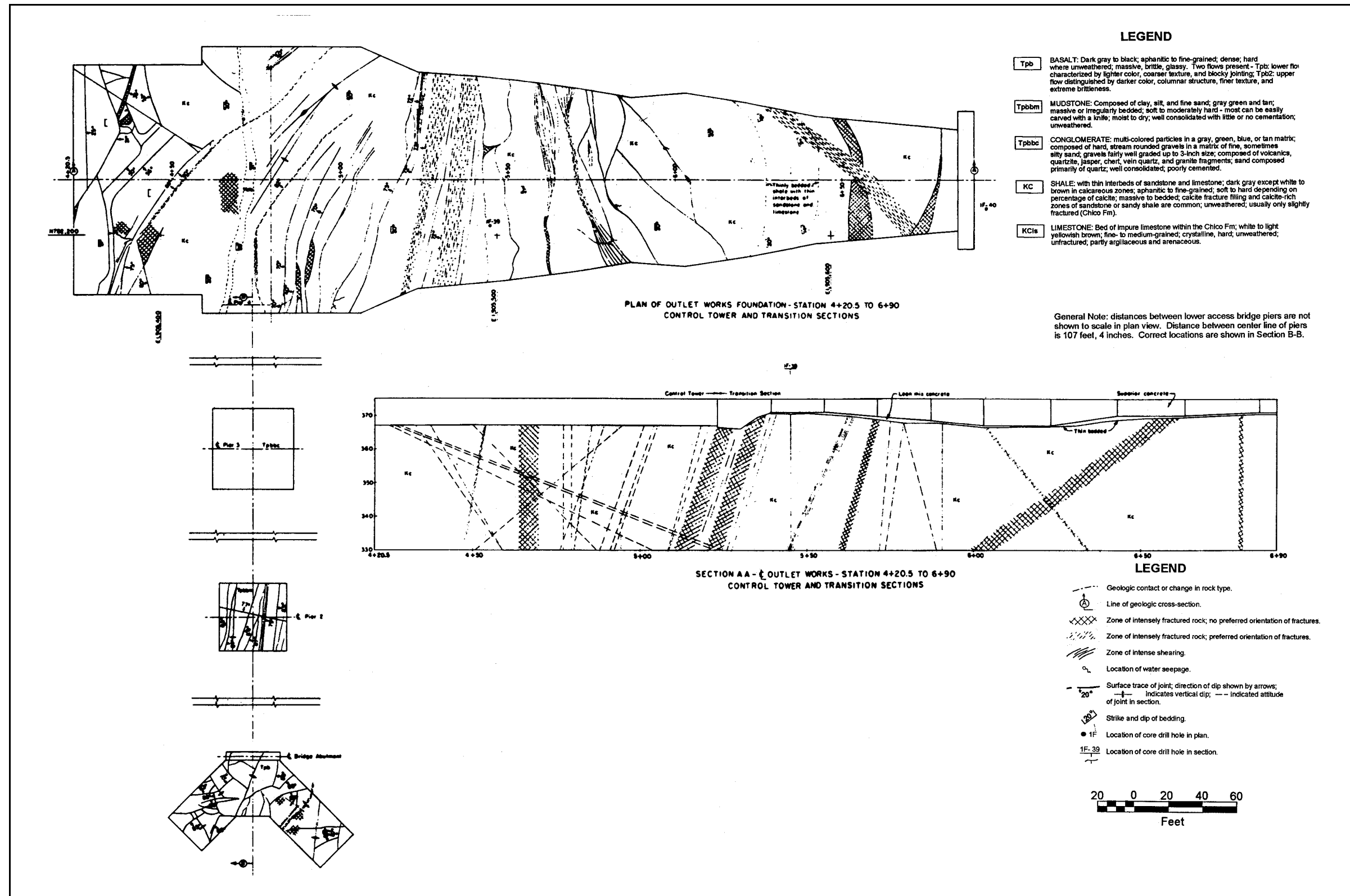
Figure B-7. Example of foundation map for concrete structure on sedimentary rocks
