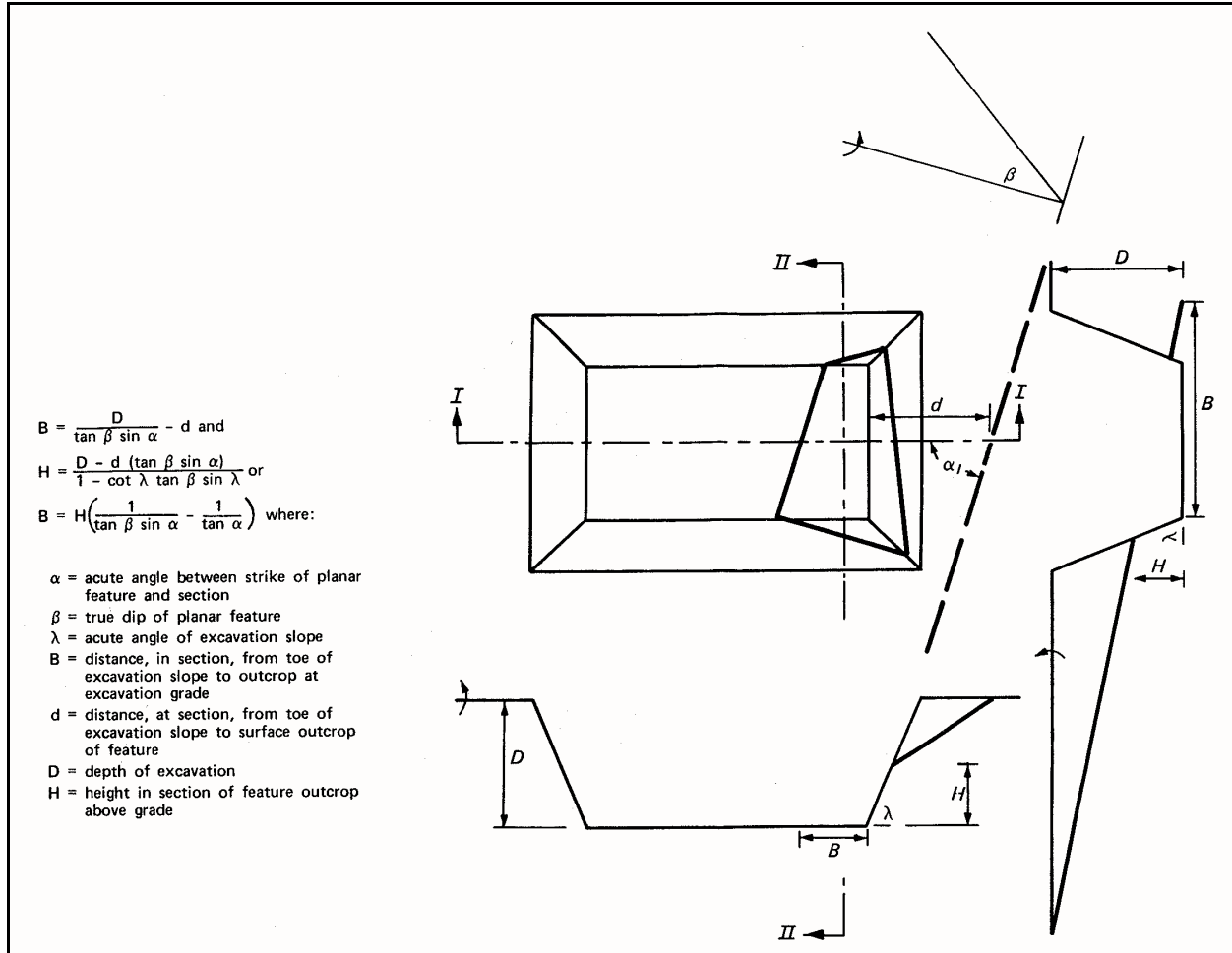
Figure B-1. Excavation plan and sections showing intersecting planar feature
