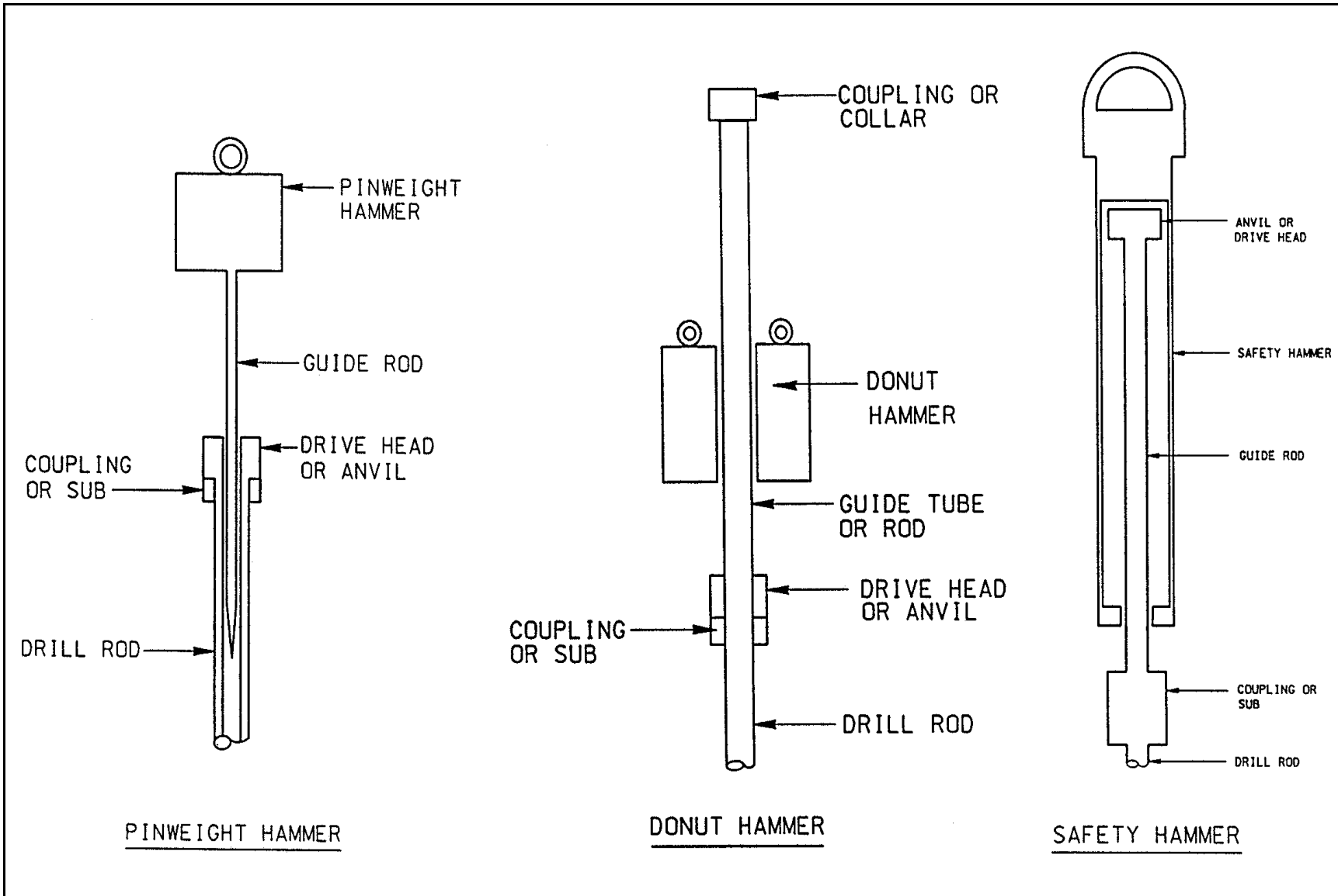
Figure G-1. Schematic drawing of the pinweight hammer, the donut hammer, and the safety hammer (after Riggs 1986)
