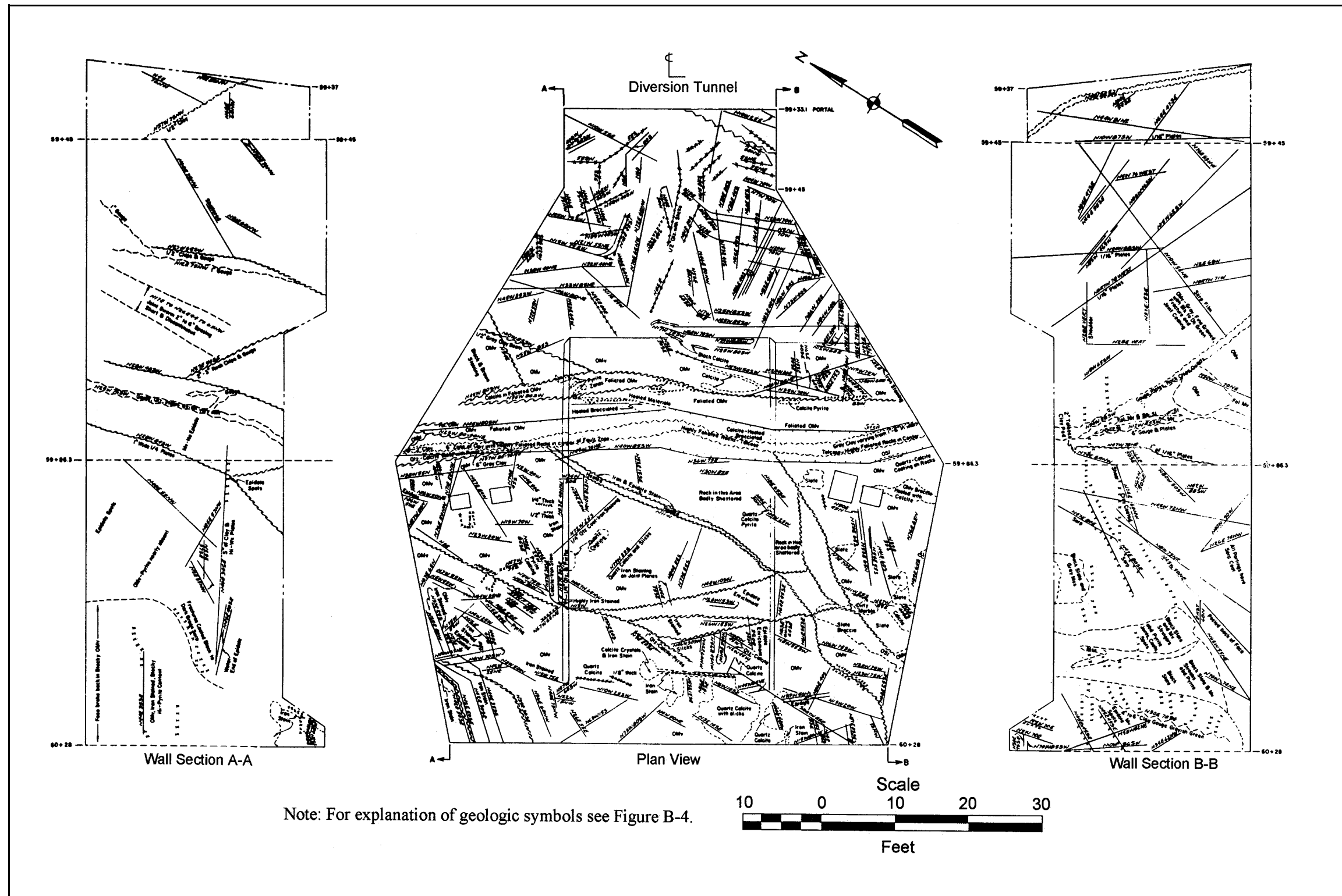
Figure B-3. Example of foundation map for structure on metamorphic rocks
