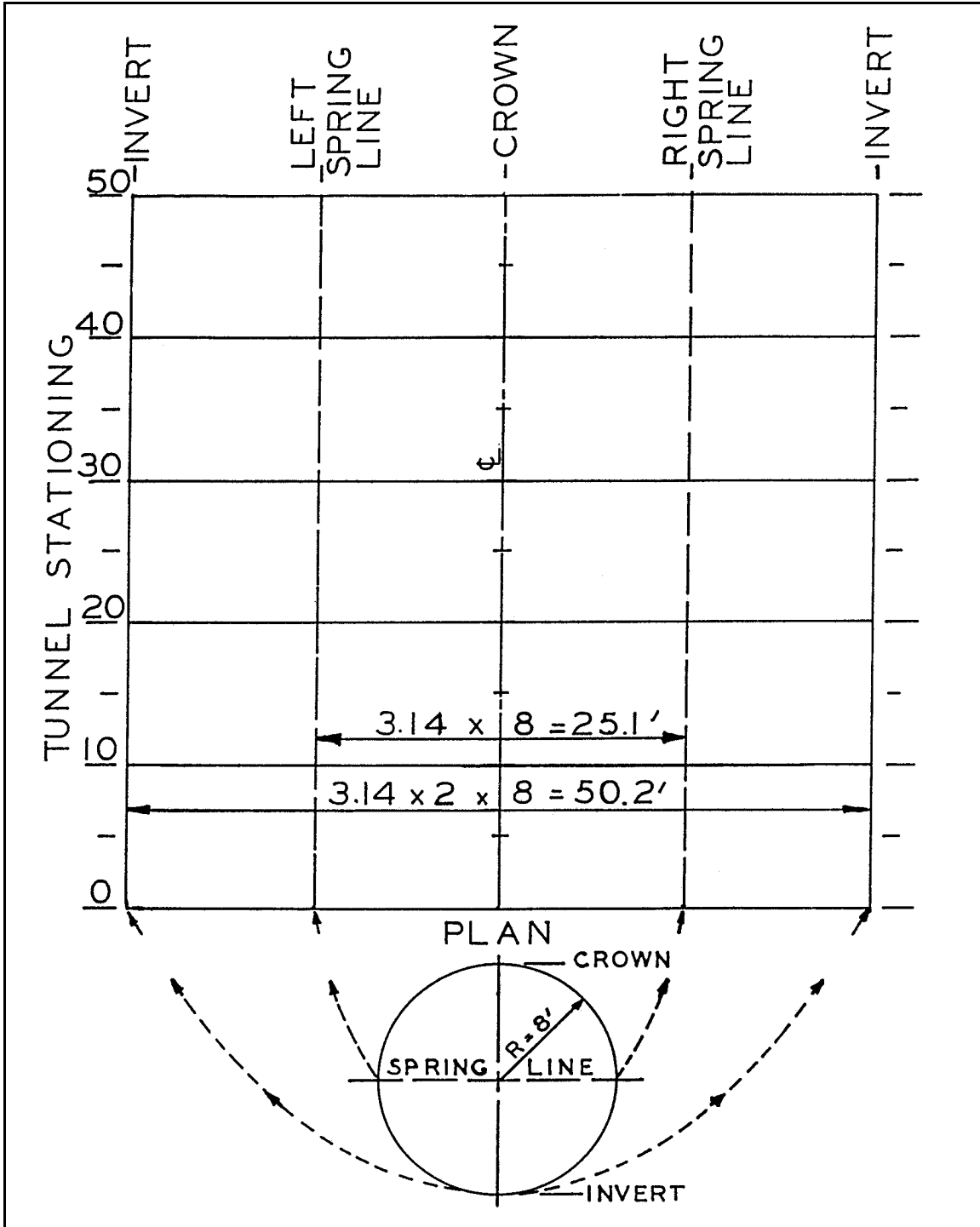
Figure C-1. Preparation of developed plan from a cylindrical cross section
