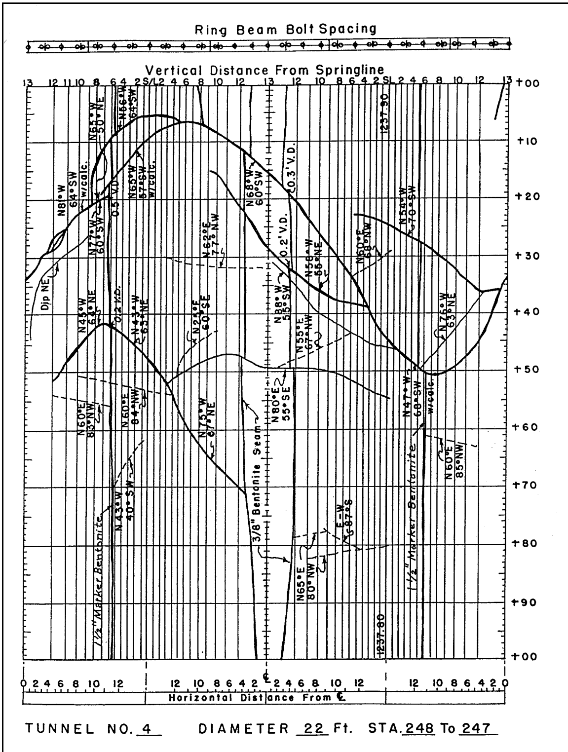
Figure C-2. Developed plan of cylindrical tunnel section Fort Randall Dam, South Dakota (note: 1 ft = 0.3 m approx.)
