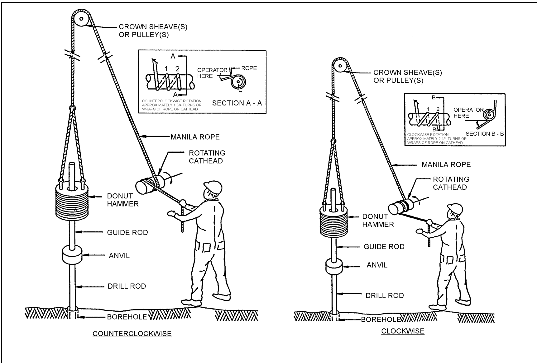
Figure G-3. Schematic drawing of the number of turns of rope on the cathead; 1-3/4 for counterclockwise rotation of the cathead, and 2-1/4 turns for clockwise rotation of the cathead
