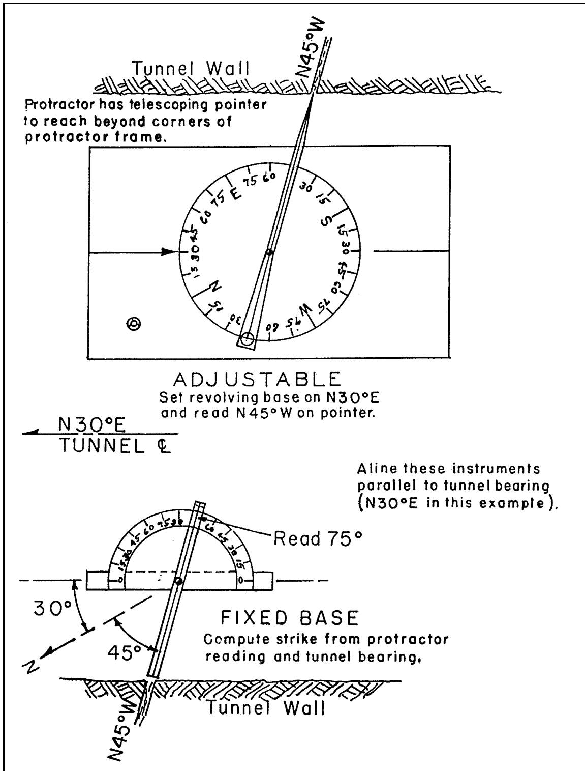
Figure C-4. Sketch of typical protractors used in peripheral geologic mapping
